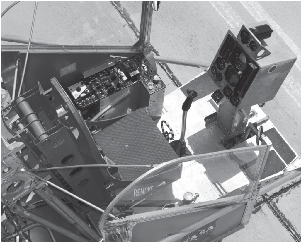
This is the original cockpit configuration of LLRV no. 1. The Plexiglas® side and front panels still are in place. The lightweight Weber ejection seat, center stick, lift-control handle, and rudder pedals are visible, as is the center-mounted instrument pedestal. (E-13115)
